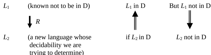
Figure 21.1 Using reduction for undecidability
