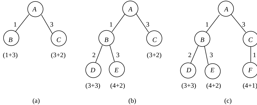
Figure 30.2 Best-first search
