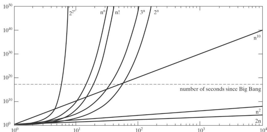
Figure 27.1 Growth rates of functions
